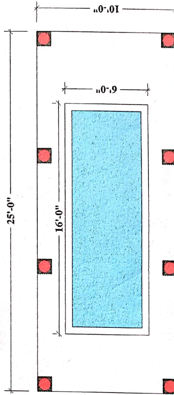
PLAN
