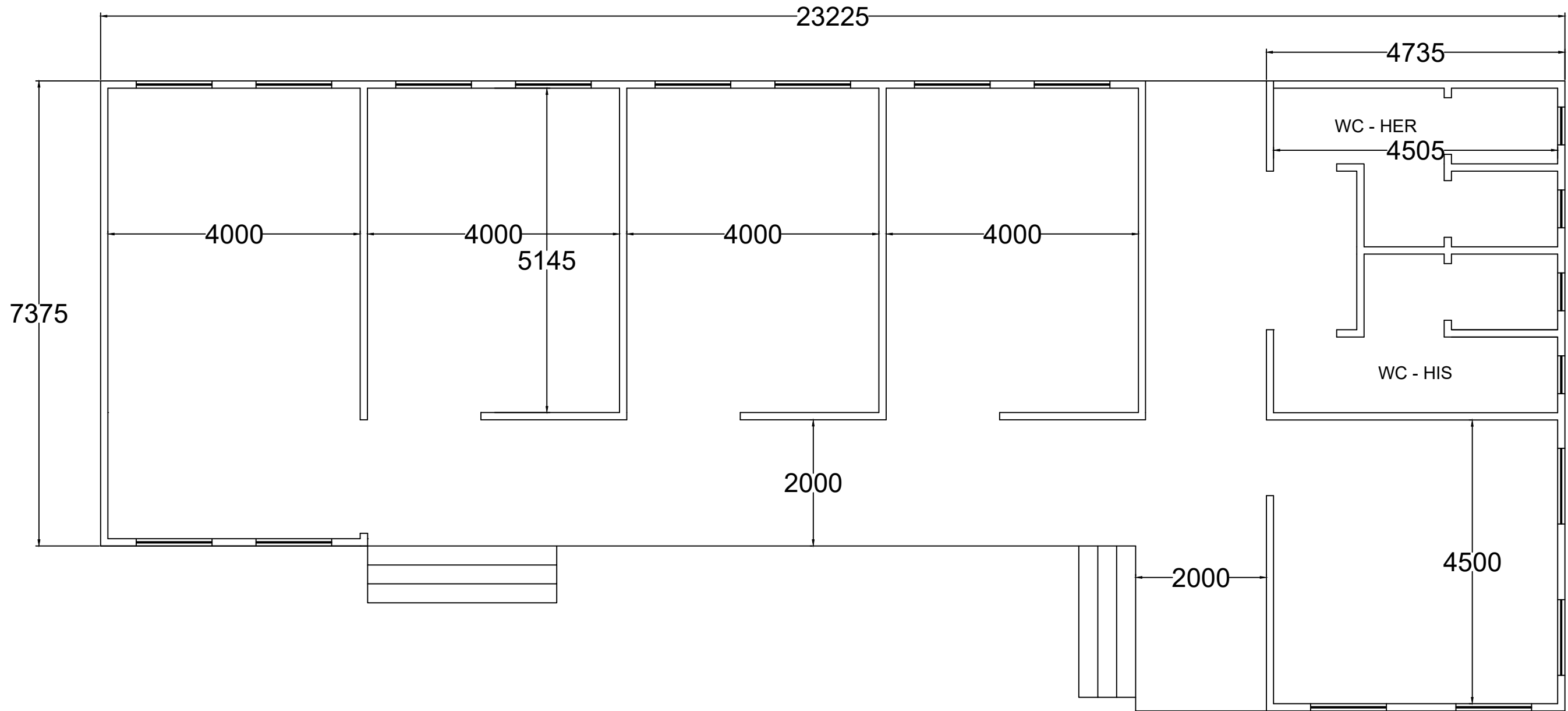
LAYOUT PLAN
