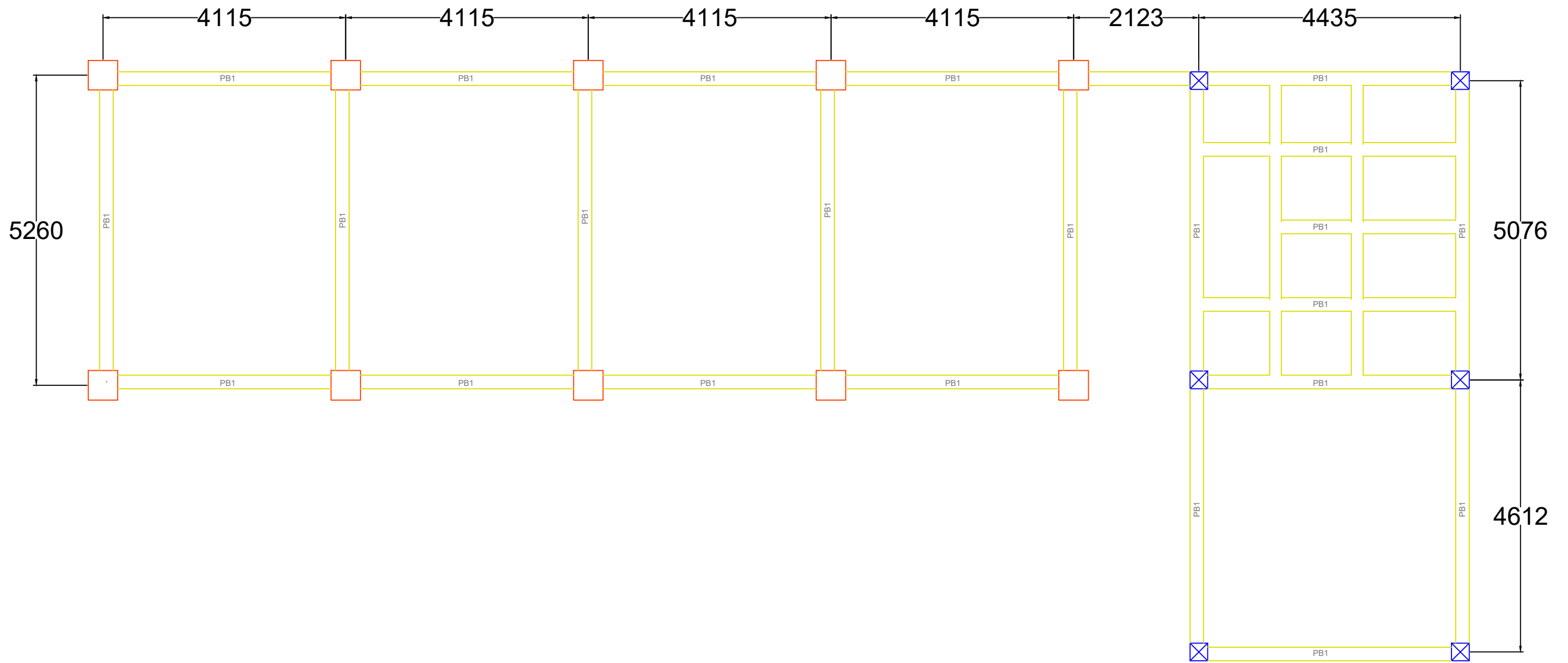
PLINTH BEAM PLAN
