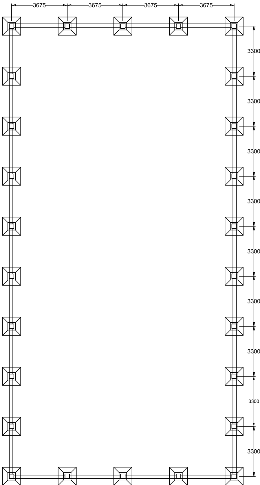
LAYOUT OF TIE BEAM & FOUNDATION
