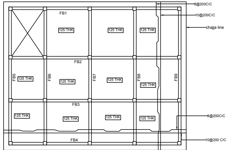
LAYOUT OF SLAB
