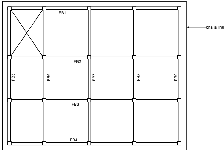
LAYOUT OF ROOF BEAM
